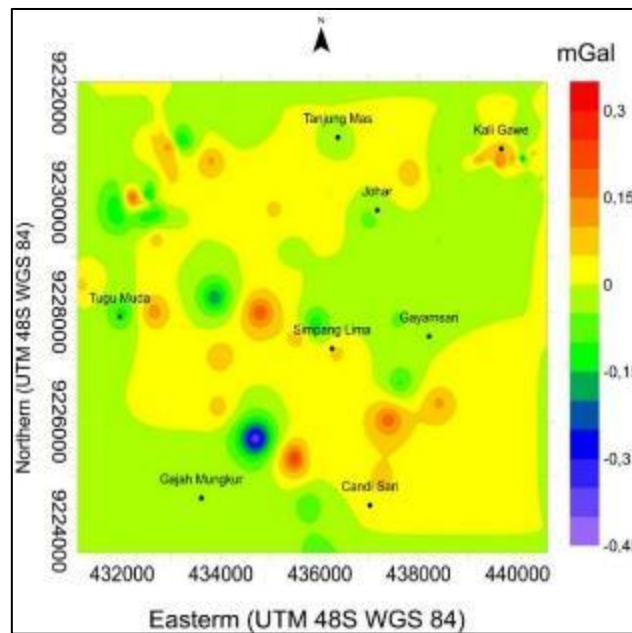
Figure 4. Complete Bouguer Anomaly (CBA) residual map results
