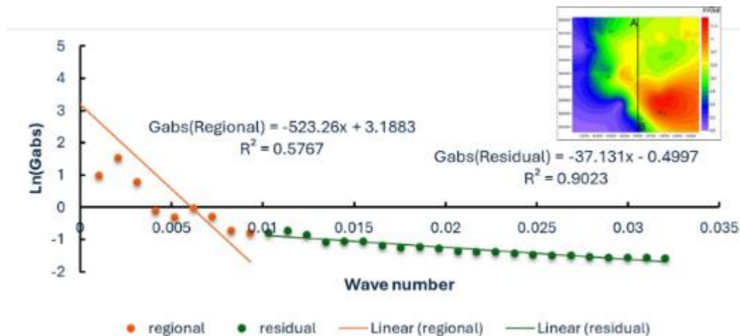
Figure 3. Separation between residual CBA and regional CBA using the spectrum analysis method
