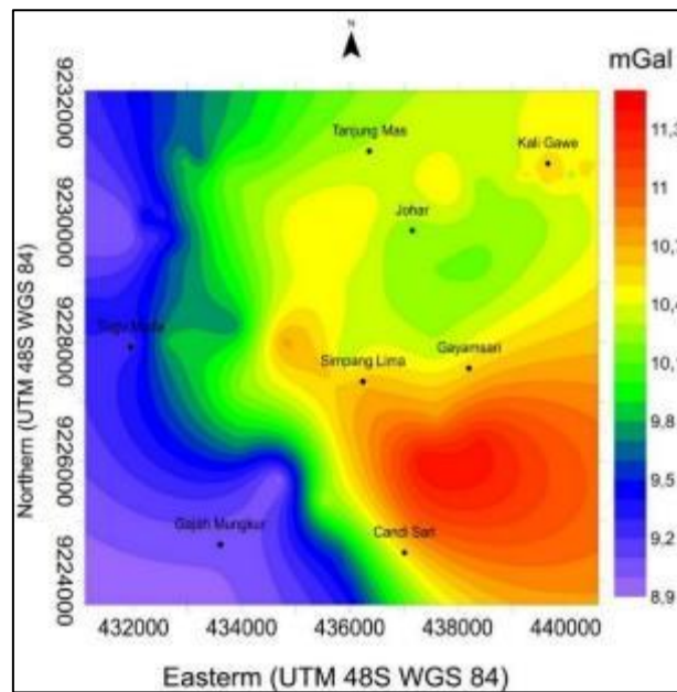
Figure 2. Complete Bouguer Anomaly (CBA) map that has undergone various correction processes
