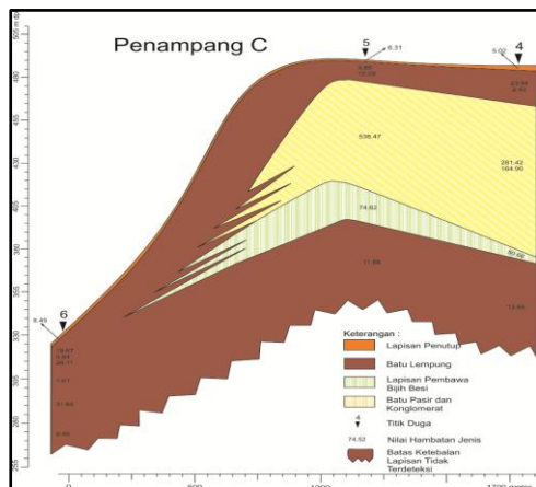
Gambar 6. Penampang C
