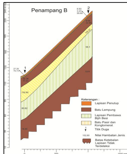
Gambar 5. Penampang B
